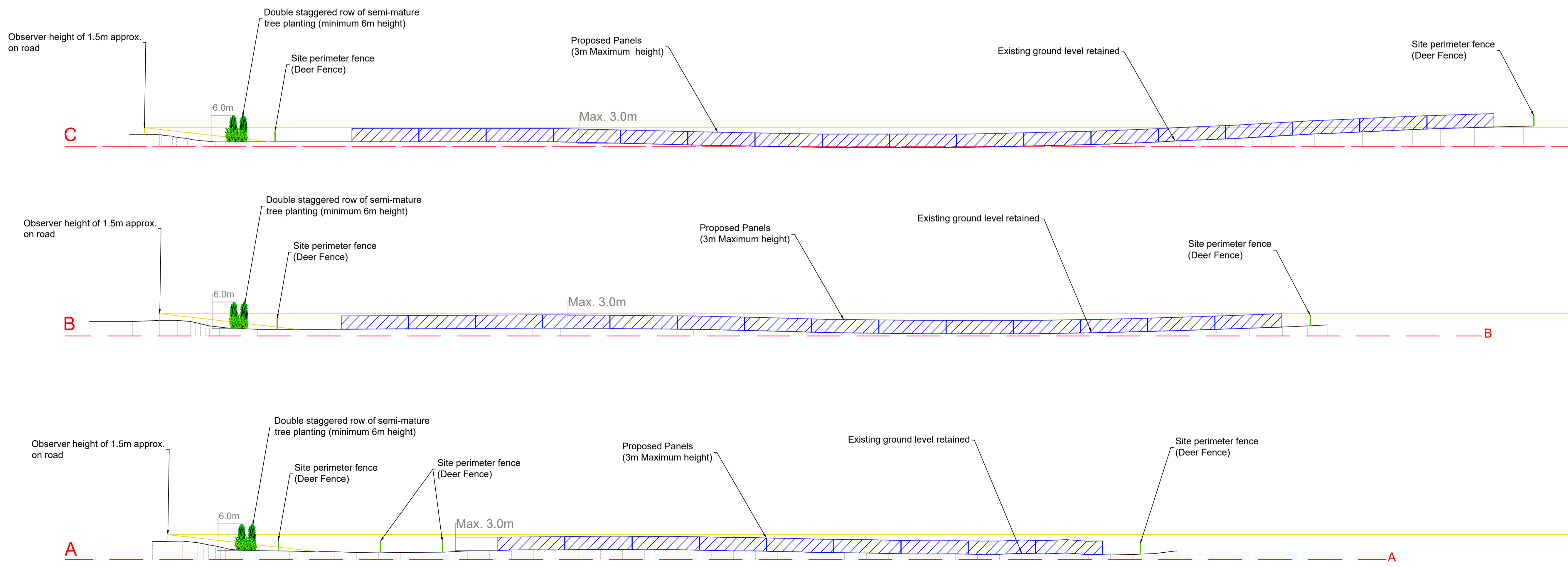
SECTION A, Section B & Section C Scale 1:500
